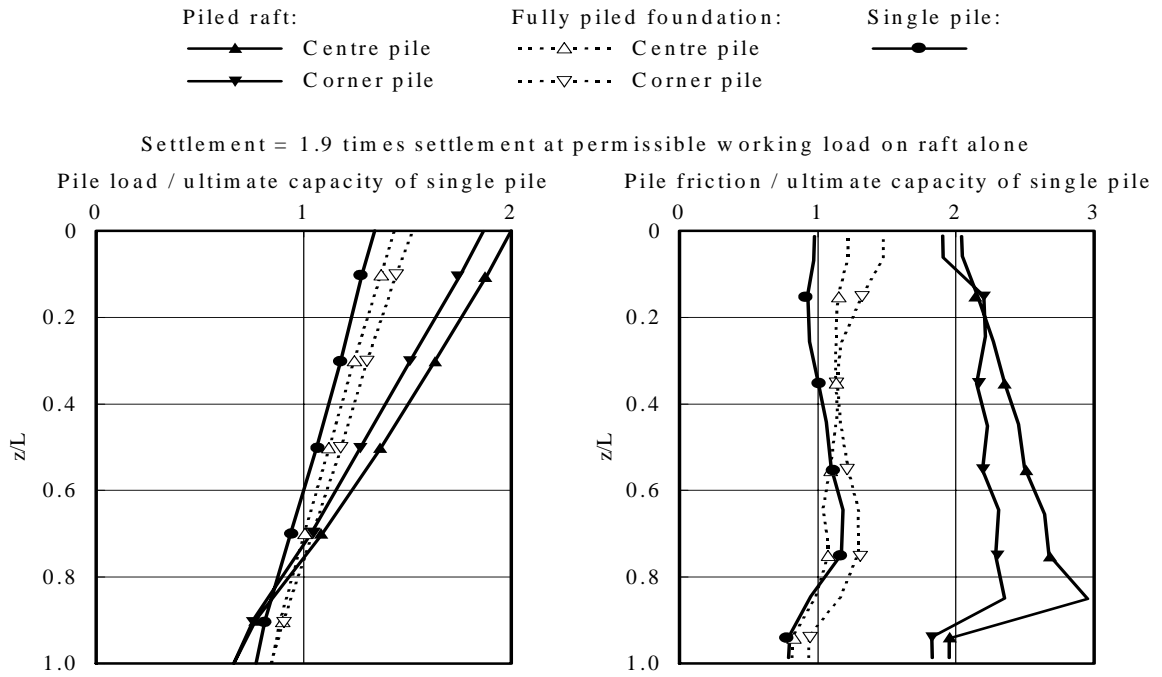
Fig.17 Distribution of the pile load and the skin friction along the pile shaft - raft with 13 piles (Katzenbach et al, 1998)
